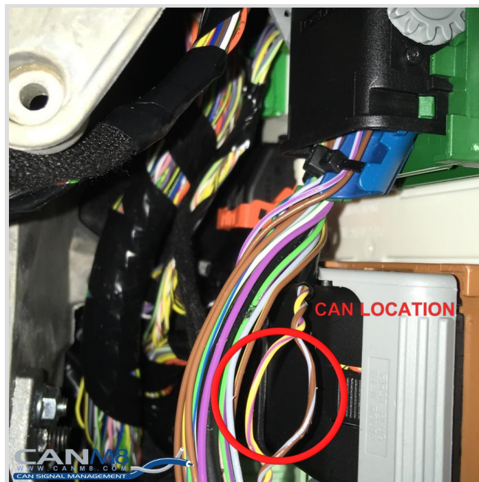
CAN Wiring (image is from below)
